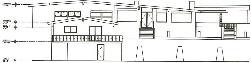
SOUTH ELEVATION SCALE: 3/16" = 1'-0"
